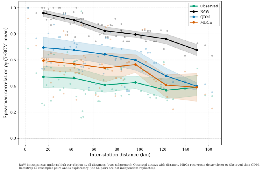
Figure 4. Inter-station Spearman correlation versus gauge separation. MBCn follows the observed distance relationship more closely than QDM, whereas raw output remains uniformly high. Bootstrap bands are exploratory because gauge pairs are not independent.
