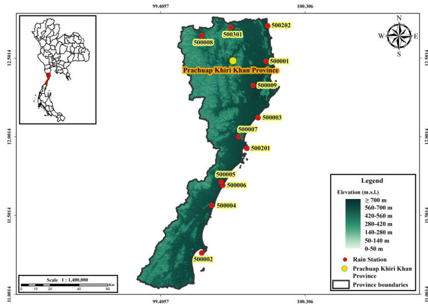
Figure 1. Location of the 12 rain gauges in Prachuap Khiri Khan Province, Thailand. Red circles mark gauge locations and labels identify the stations. Background shading represents elevation classes, and the inset shows the province's location within Thailand.
