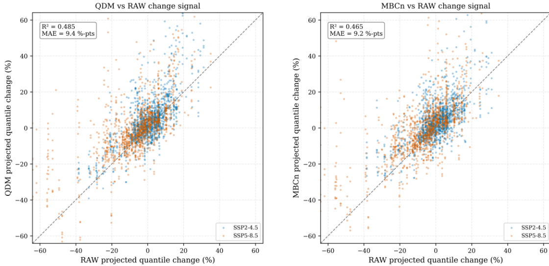
Figure 6. Raw versus corrected projected change in wet-day quantiles for every gauge, model, pathway, and future period. QDM and MBCn preserve the model-projected quantile-change signal to a similar degree.
